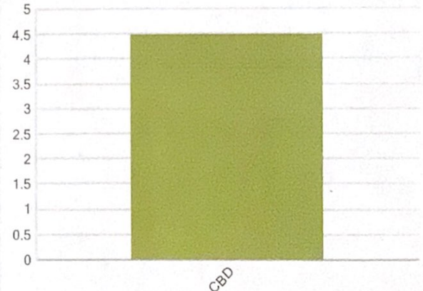
Cannabinoids (% weight)
